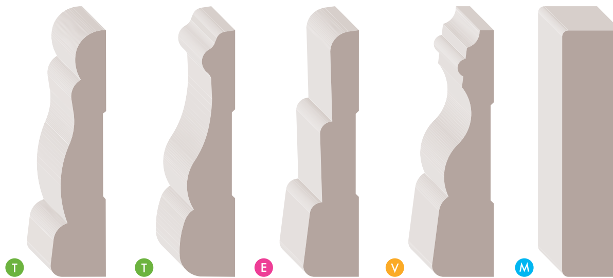
00603 9/16" x 2-1/2" FJP • SP 7', 14' 7' 00607 9/16" x 2-1/2" FJP • SP 7', 14' 7', RL 00630 9/16" x 2-1/2" FJP 7' 00635 5/8" x 2-1/2" VIR 7', RL 02183 5/8" x 2-1/2" DECO 8'
