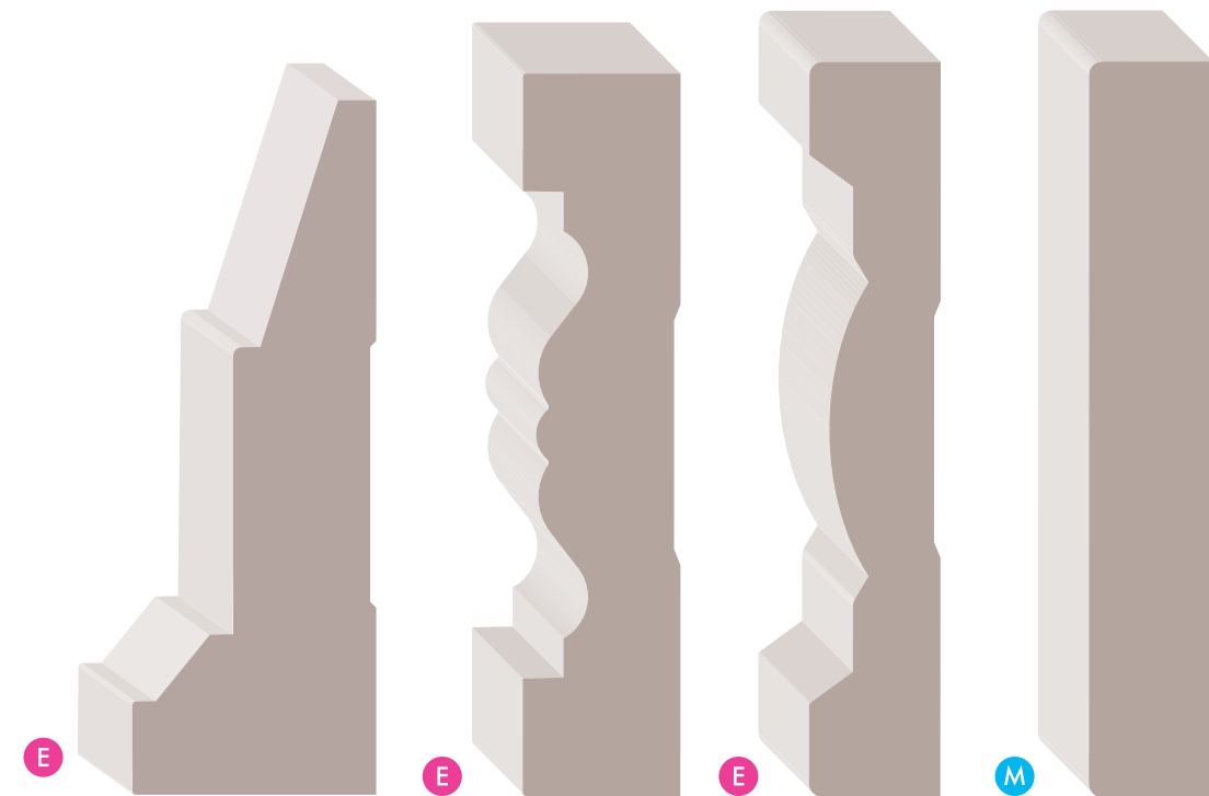
01693 1-1/8" x 3-1/4" PMDF 15' CR690 3/4" x 3-7/16" PMDF 8', 16' 03652 5/8" x 3-1/2" PMDF 7'1", 14'3" 02184 5/8" x 3-1/2" DECO 8'
