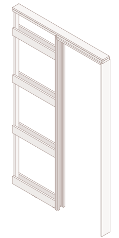
PD132 32" x 80" (With 4-9/16" Jamb)
