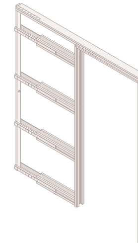
PD724 24" to 36" x 80" (Adjustable) (With 4-5/8" Jamb)
