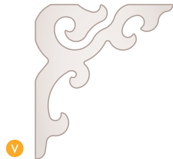
GB001 Porch Bracket 14-3/4" x 16-9/16" PVC 3/4"
