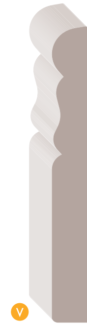
07622 3/8" x 3-1/8" PMDF • DECO • FLEX 8', 12', 14' 8', 12' RL
