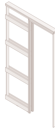
PD124 24" x 80" (With 4-9/16" Jamb)
